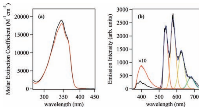
Figure 6. (a) Absorption spectra of the [\text{Yb}(\text{5LIO-Me-3,2-HOPO})_2] (red) and [\text{Yb}(\text{H}(2,2)\text{-Me-3,2-HOPO})] (black) complexes in 0.1 M aqueous TRIS buffer, pH 7.4. (b) Emission spectra ( \lambda_{\text{ex}} = 345 \text{ nm} ) at room temperature (red, \times 10 ) and 77 K (black) of the [\text{Gd}(\text{5LIO-Me-3,2-HOPO})_2]^- complex measured in a 1:1 (v/v) EtOH/MeOH glassing solvent, and corresponding fit (blue) to a series of overlapping Gaussians to evaluate the zero phonon transition.
