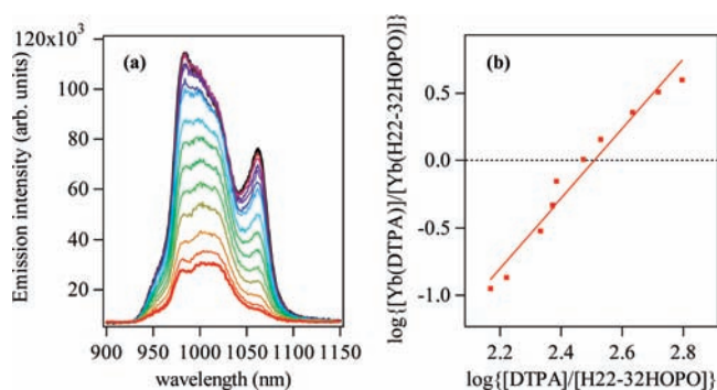
Figure 4. (a) Luminescence spectra (left) for solutions of [\text{Yb}(\text{H(2,2)-Me-3,2-HOPO})] (ca. 1.5 \mu\text{M} in 0.1 \text{ M TRIS} at \text{pH } 7.4 ; black line) and after addition of up to about 500 equiv of DTPA (red). (b) Double log plot (right) of equilibrium metal complex concentrations \log \{[\text{Yb}(\text{DTPA})]/[\text{Yb}(\text{H(2,2)-Me-3,2-HOPO})]\} determined from luminescence spectra versus equilibrium concentrations of \log \{[\text{DTPA}]/[\text{H(2,2)-Me-3,2-HOPO}]\} and corresponding fit used to evaluate equal speciation between H(2,2)-Me-3,2-HOPO and DTPA (i.e., 50% [\text{Yb}(\text{DTPA})] ) at about 0.013 \text{ mM} , which corresponds to a \text{pYb} = 21.9 (1) for the [\text{Yb}(\text{H(2,2)-Me-3,2-HOPO})] complex).
